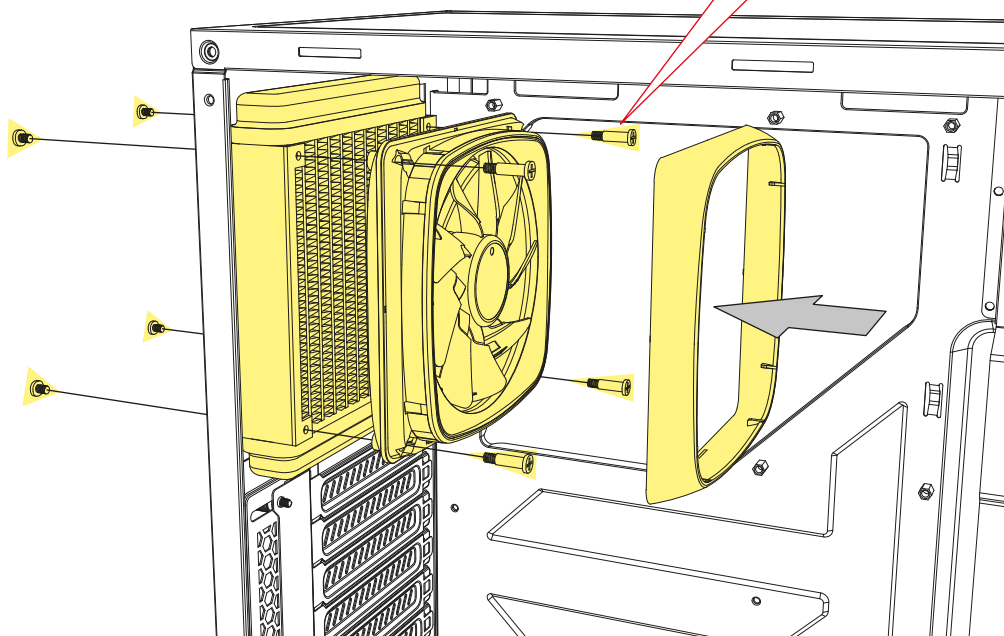
120 mm Radiator
