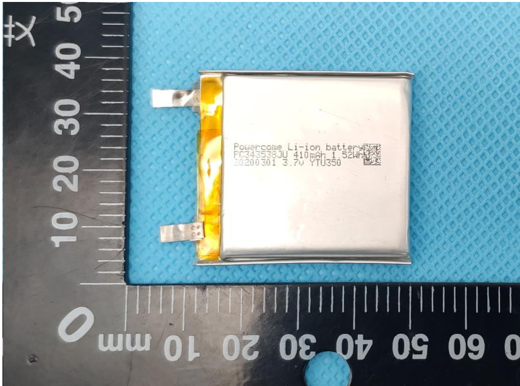
Cells /电芯 (PC343538JU 3.7V 410mAh 1.52Wh)
