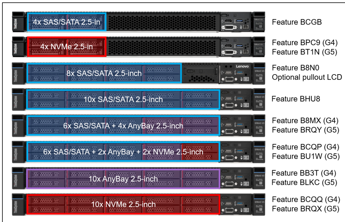
Figure 12. SR645 V3 front drive bay configurations - 2.5-inch drive bays without front PCIe slot support
