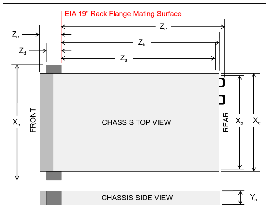
Figure 26. Server dimensions
