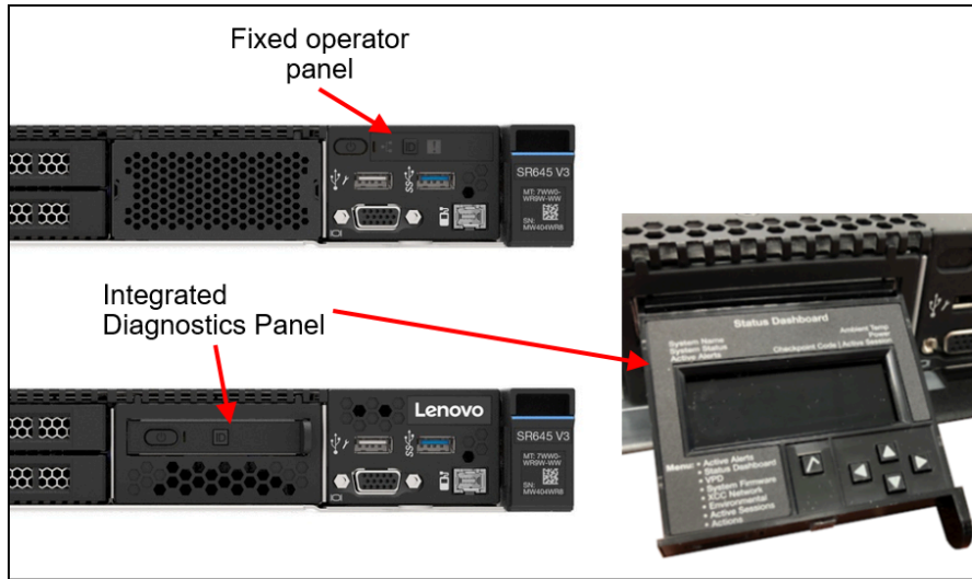
Figure 22. Operator panel choices for the EDSFF and 8x 2.5-inch drive bay configurations
