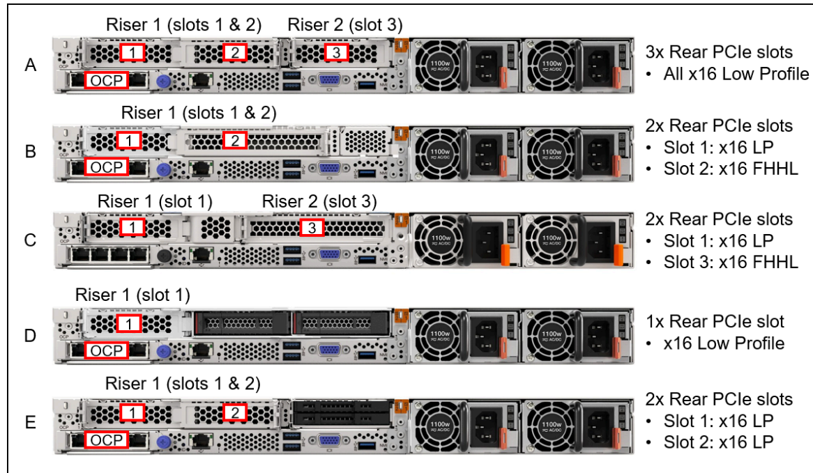
Figure 16. SR645 V3 rear slot configurations
