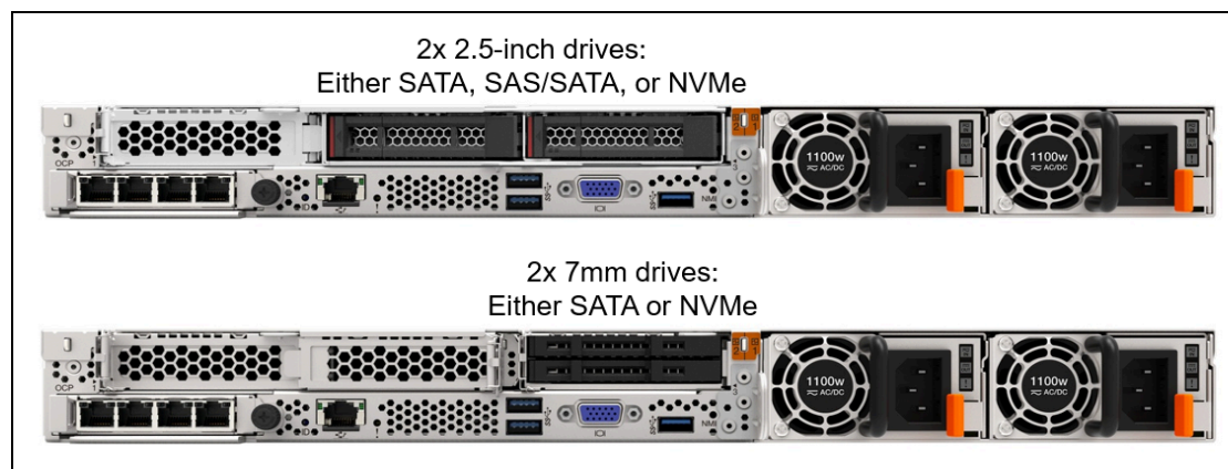
Figure 14. Rear drive bay configurations
