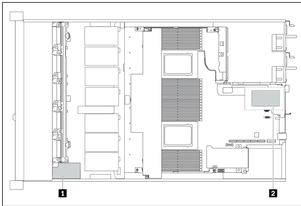
Figure 15. Location of the supercaps in the SR645 V3
