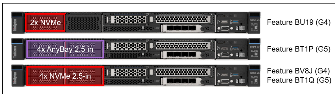
Figure 13. SR645 V3 front drive bay configurations - 2.5-inch drive bays with front PCIe slot support
