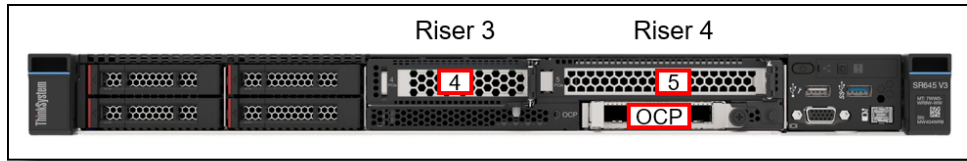
Figure 17. SR645 V3 front slots
