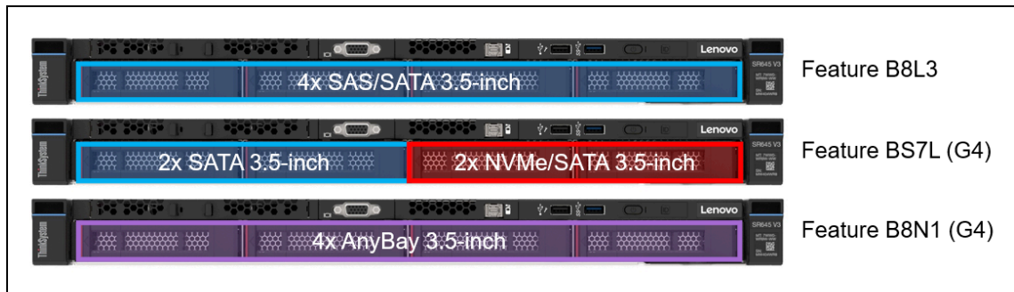
Figure 10. SR645 V3 front drive bay configurations - 3.5-inch drive bays
