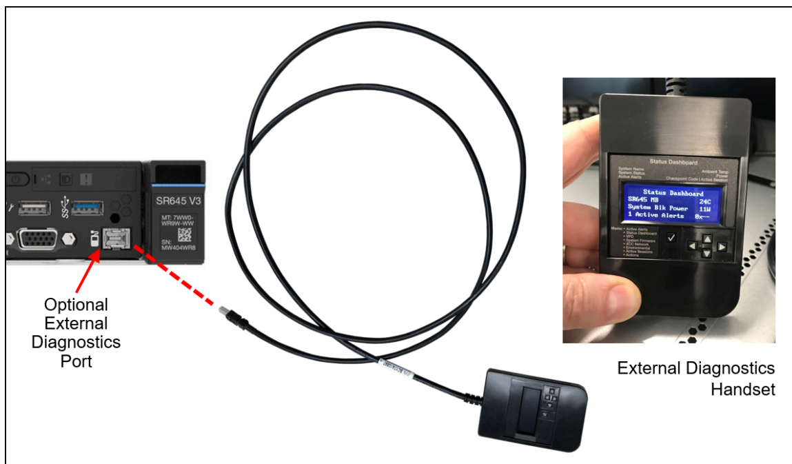
Figure 23. External Diagnostics Handset
