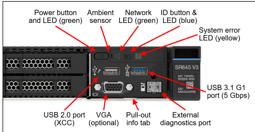
Figure 21. Front operator panel
