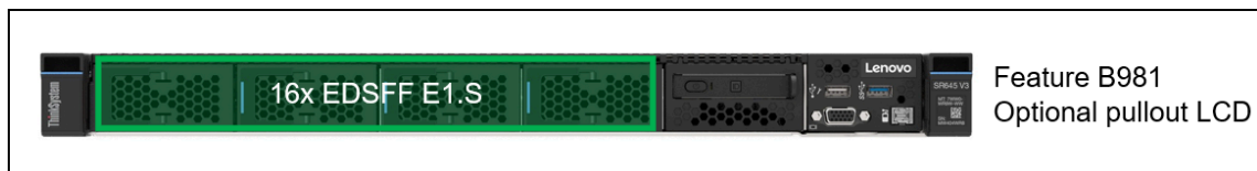
Figure 11. SR645 V3 front drive bay configurations - EDSFF E1.S drive bays
